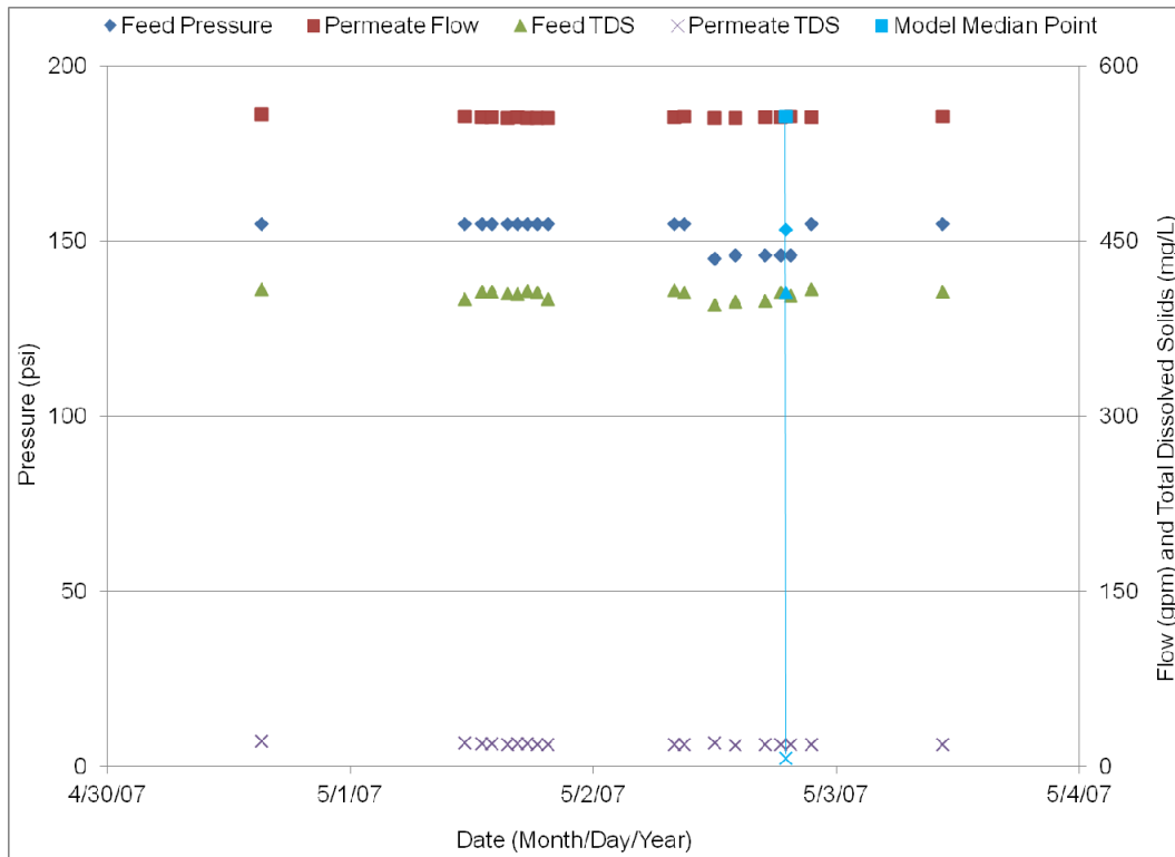
Figure 4-11. Actual start-up (time series) vs. model data (median points emphasized with vertical line) comparison for Hardinsburg Train A.
